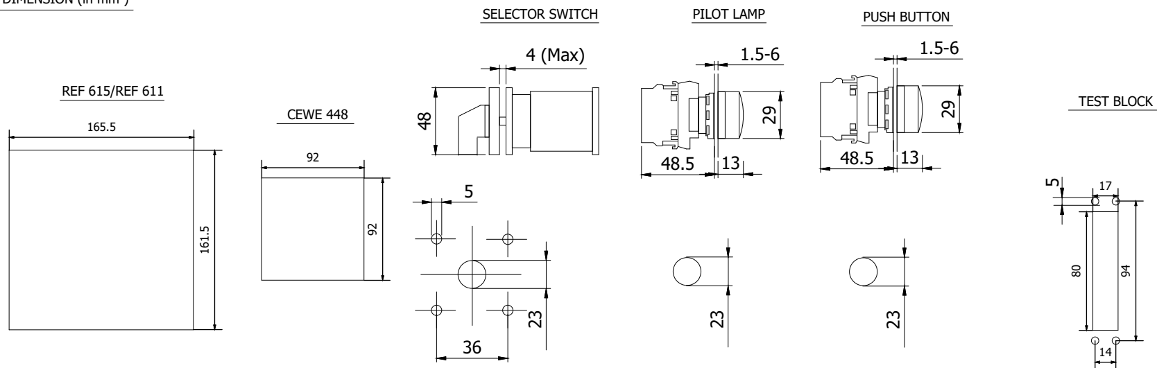
CUT OUT DIMENSION (in mm )
